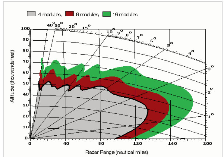
ASR-L free-space coverage (Low-Beam) with 4, 8, and 16 module transmitters (5 sq. m target, 4-Pulse MTD, 0.8 probability of detection)
